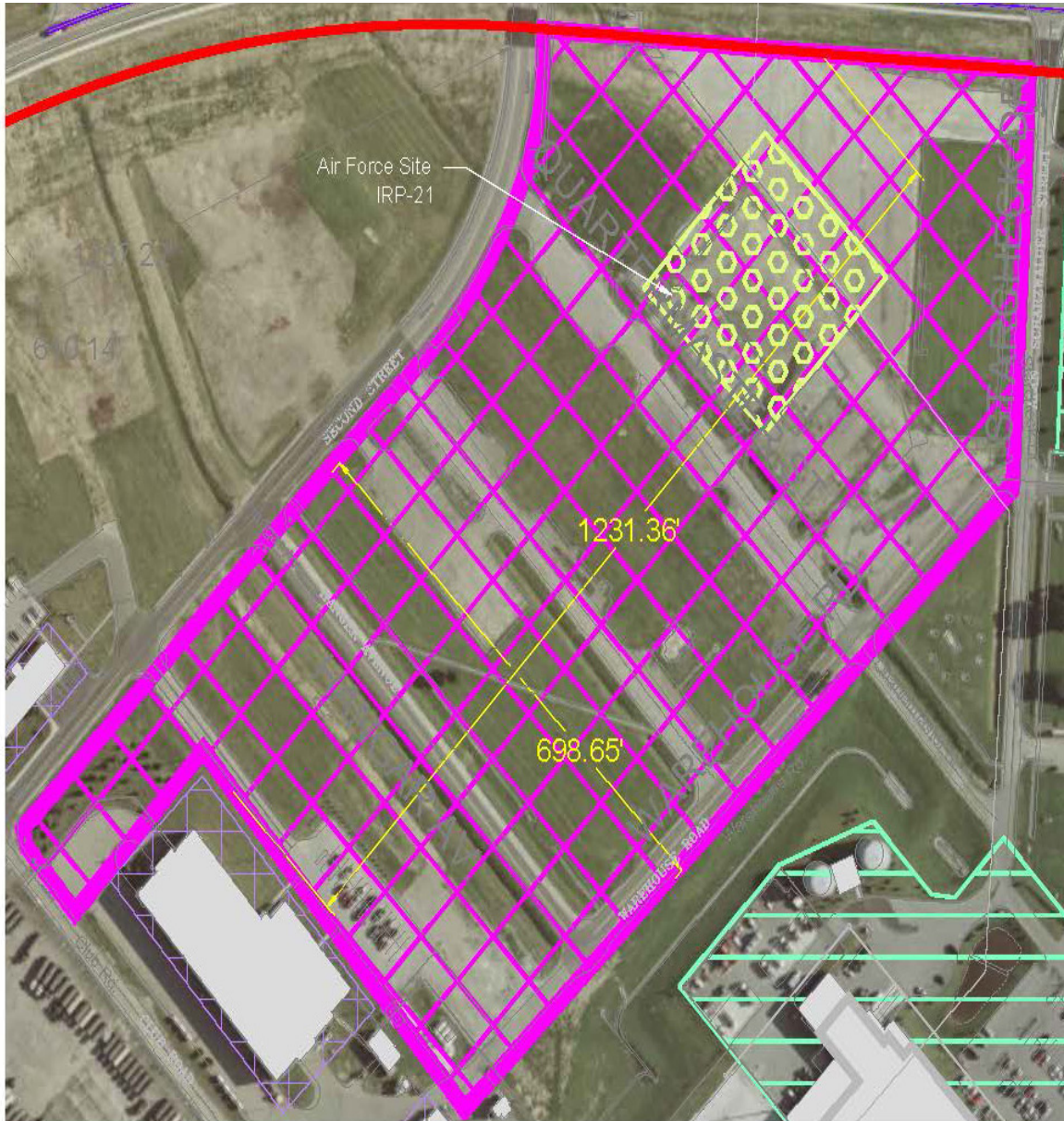
Second St. – Parcel #16 21 Ac. ± 1" = 200'
