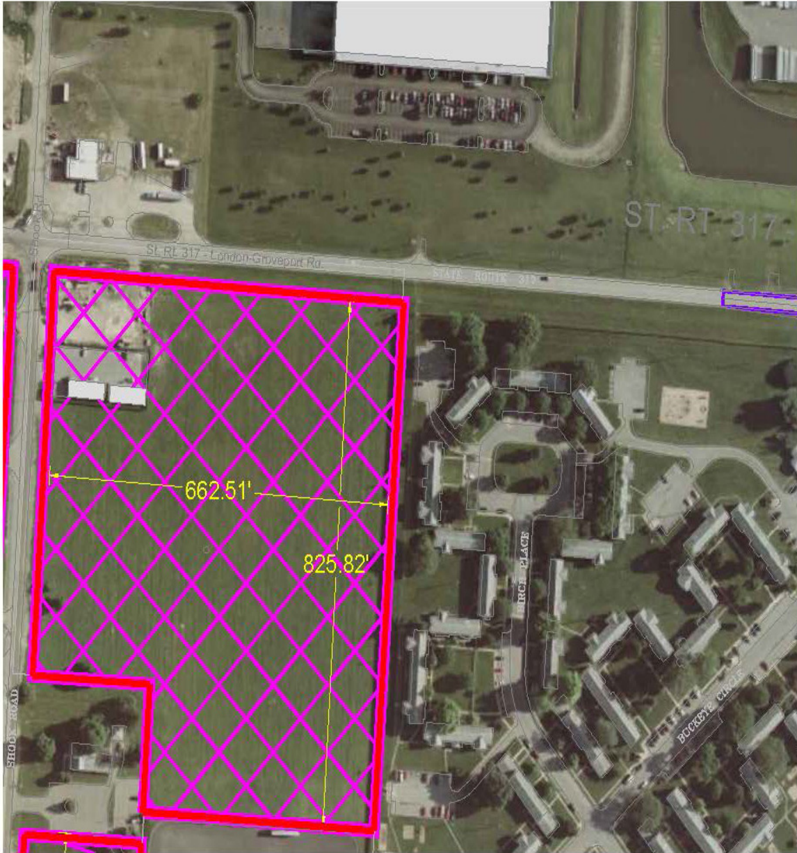
St. Rt. 317- London-Groveport Rd. – Parcel #13 12 Ac. ± 1" = 200'
